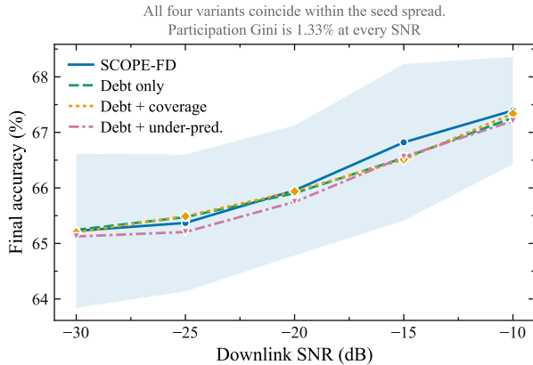
Fig. 5. Downlink SNR sweep on FMNIST at N = 30 , K = 5 over three seeds. Shaded bands are one standard deviation.
